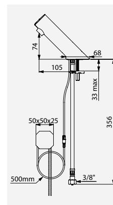
TEMPOMATIC 5 tap, mains supply Ref. DELABIE: 44900015
