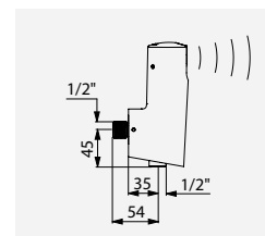
TEMPOMATIC 4, angled valve Ref. DELABIE: 479411
