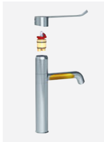
Mechanical basin mixer with swivelling spout Ref. DELABIE: 2564T1
